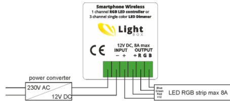
Diagram 1: LightBox to RGB color LED strip connection
